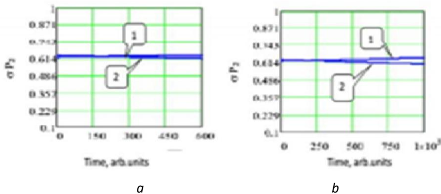
Fig. 1. Calculated time dependencies of the quantities: \square_1 P_{21} (curves 1) and \square_2 P_{22} (curves 2) on the graphs (a) and (b) at various analytic model constants: A_1 = 2.1, t^*_1 = 8 \square 10^4 \text{ arb. units} , \square^*_1 = 1.2 \text{ MPa} ; A_2 = 10^{4.9}
