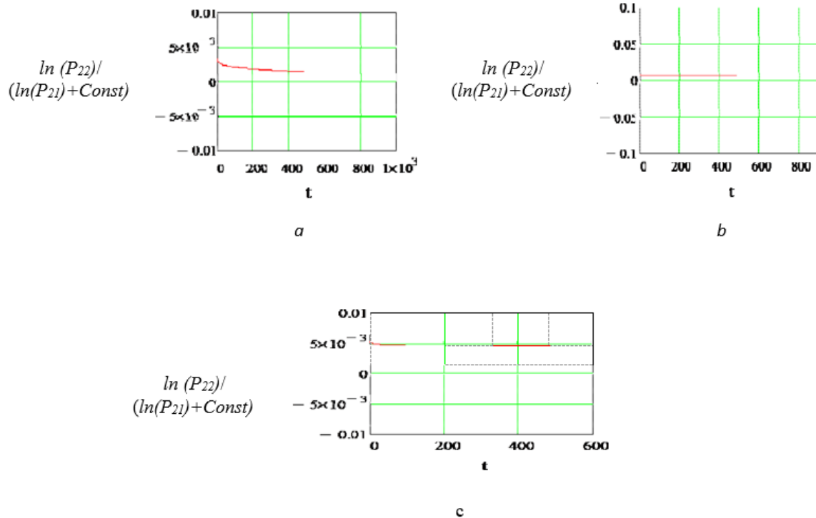
Fig.2. Calculated time dependencies of the quantities \ln(P_{22}) and \ln(P_{21}) + \text{Const} in the form of their relation \ln(P_{22})/(\ln(P_{21}) + \text{Const}) at various the analytic model constants: a) A_2 = 10^9 , t^*_2 = 0.09 arb.units, A_1 = 3 , t^*_1 = 200 arb.units, \text{Const} = 900 ; b) A_2 = 10^{18} , t^*_2 = 0.03 arb.units, A_1 = 3 , t^*_1 = 200 arb.units, \text{Const} = 500 ; c) A_2 = 10^{18} , t^*_2 = 0.09 arb.units, A_1 = 5 , t^*_1 = 200 arb.units, \text{Const} = 700
